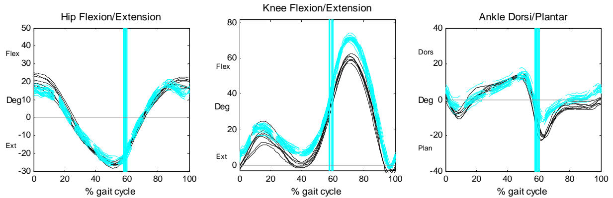
Figure: Hip, knee and ankle sagittal plane kinematics measured by the two systems: in black-solid the 7 indoor trials from CAST (Vicon 460), and in cyan-dash the 26 outdoor trials from OutWalk (Xsens MTx).
